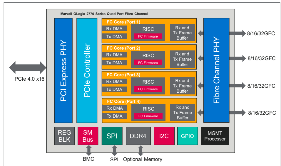
Figure 1. 2770 Series Adapters Block Diagram
